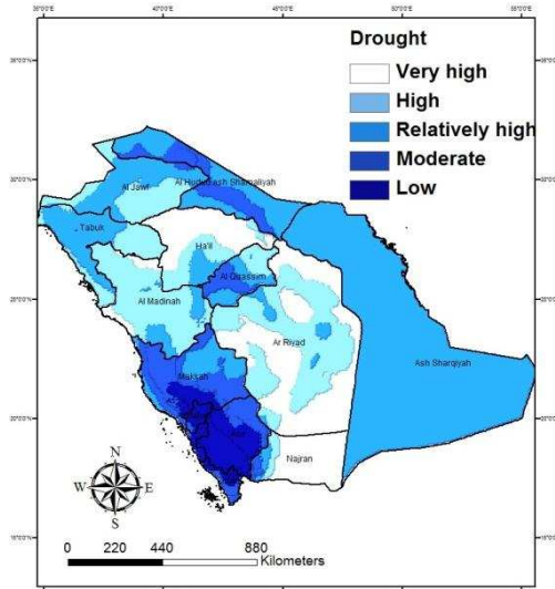
Fig. 3. The classification based on drought conditions
